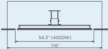
MINIMUM CAVITY FOR 4500W
