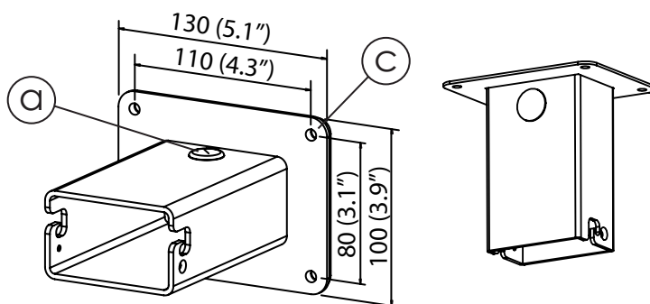
Wall mount
