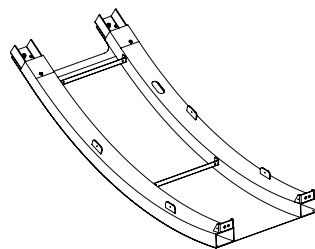
Front Assembly
