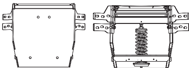
ALTERNATE HINGE
