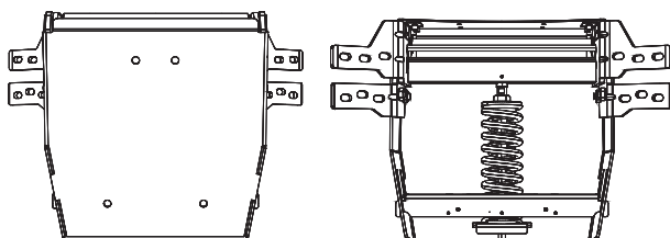
CHARNIÈRE ALTERNATIVE
